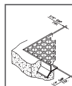
25mm grating: PN# 1617910 Install 25mm side vertical
