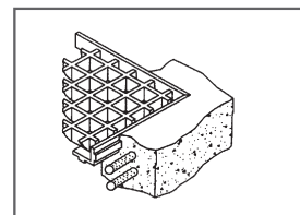
25mm grating: PN# 1617910 Install 25mm side vertical
